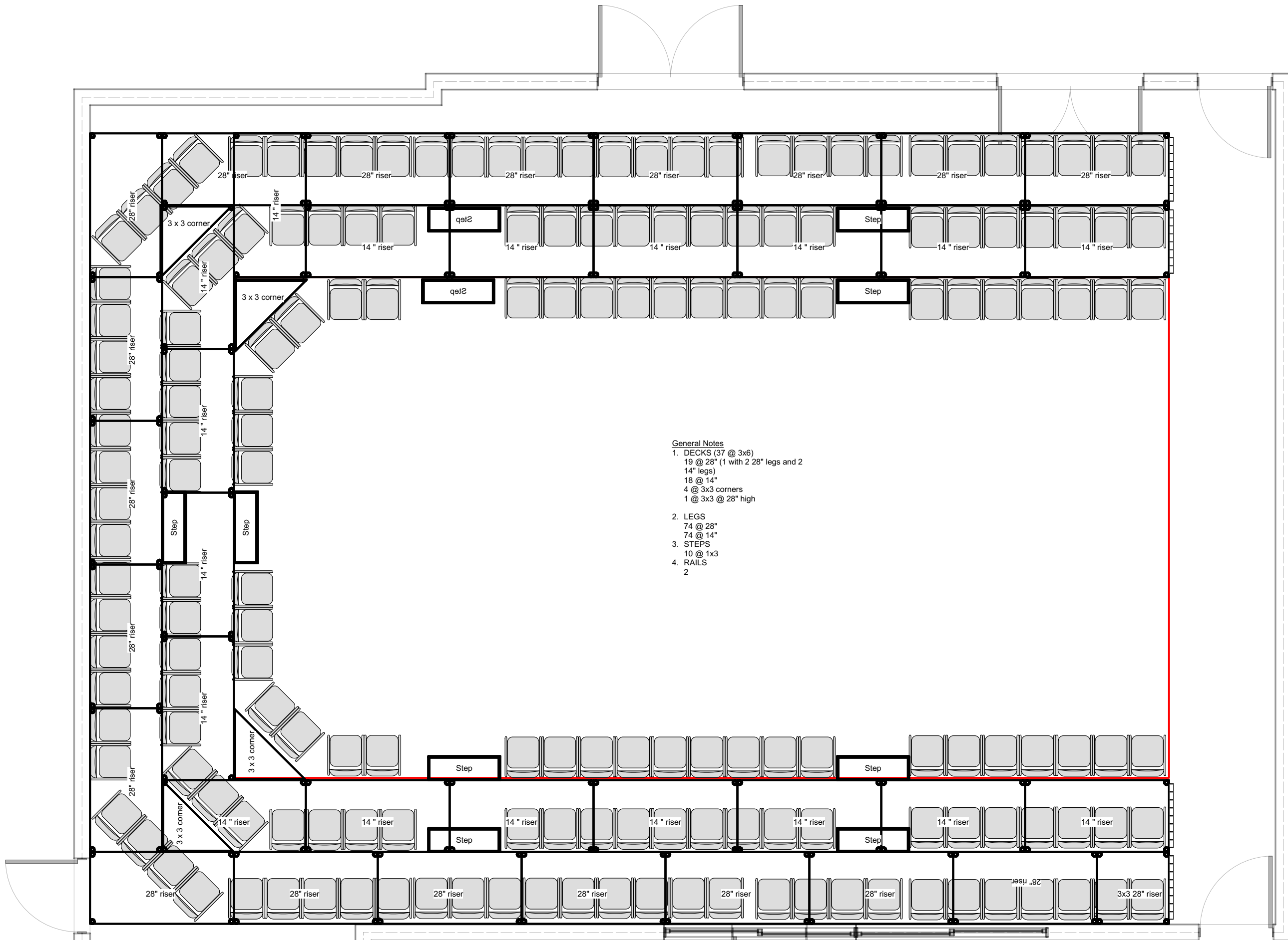
1 THRUST SEATING LAYOUT Scale: 1/4" = 1'-0"
